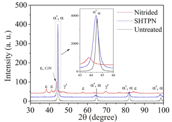
Fig. 5. X-ray diffraction pattern of untreated, plasma nitrided and SHTPN samples of AISI 409.
