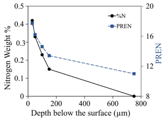
Fig. 4. The relationship between the PREN, the depth and nitrogen content for the obtained AISI 409 steel after SHTPN.
