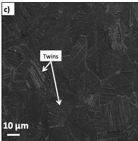
Fig. 1. SEM micrographs of the specimens annealed at (a) 700°C, (b) 900°C, (c) 1100°C for 150 min; %50 cold-rolled Fe-24Mn-0.6C high-manganese steel.
