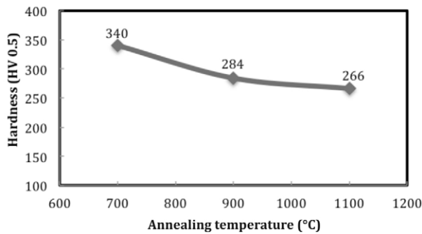
Fig. 6. Vickers hardness values of specimens annealed at 700, 900, 1100 °C and of as-rolled specimen.
