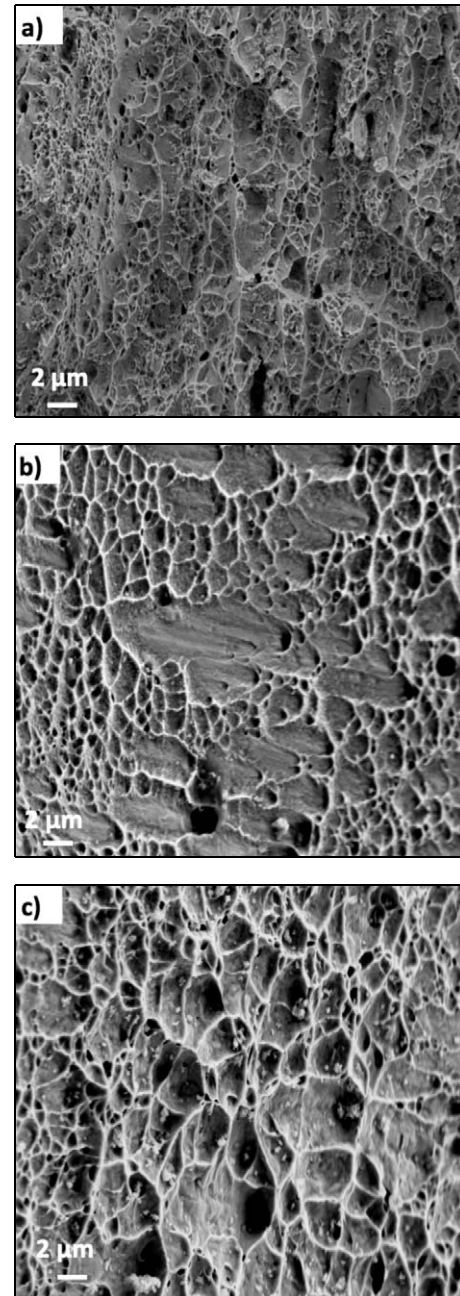
Fig. 5. SEM micrographs of the fracture surface of specimens annealed at (a) 700°C, (b) 900°C, and (c) 1100°C for 150 min; %50 cold-rolled Fe-24Mn-0.6C high-manganese steel.
