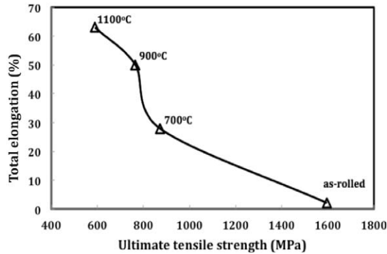
Fig. 4. The effect of annealing temperature on ultimate tensile stress – total elongation balance of samples.
