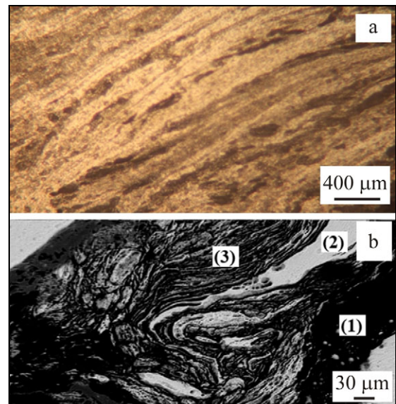
Fig. 5. a) Image obtained from the optical microscope and b) image of the welded sample obtained from scanning electron microscope in the weld zone.
