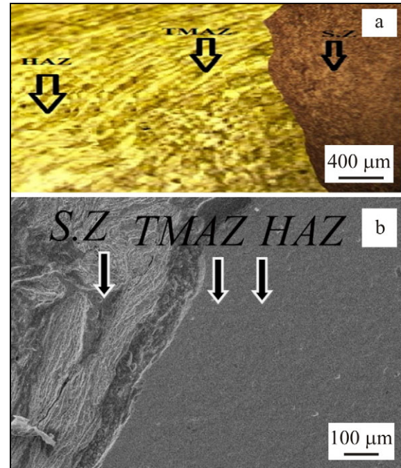
Fig. 3. a) Image obtained from the optical microscope and b) image of the welded sample obtained from scanning electron microscope in aluminum 5083 zone.
