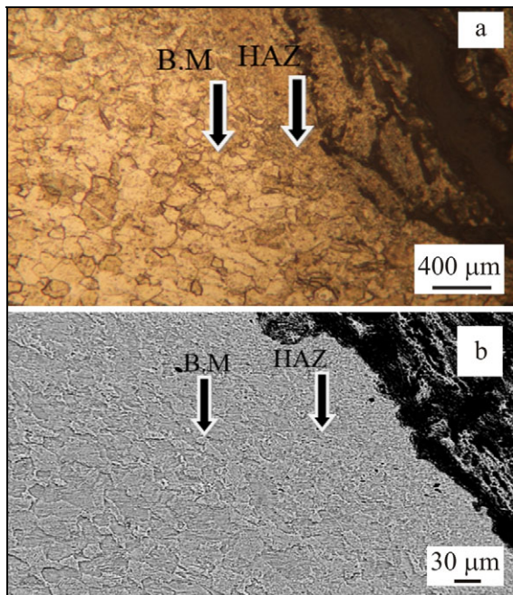
Fig. 4. a) Image obtained from the optical microscope and b) image of the welded sample obtained from scanning electron microscope in pure titanium zone.
