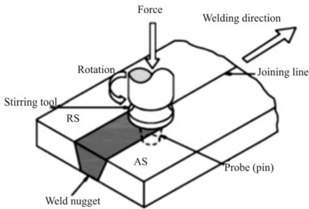
Fig. 1. Schematic presentation of FSW technique [3].
