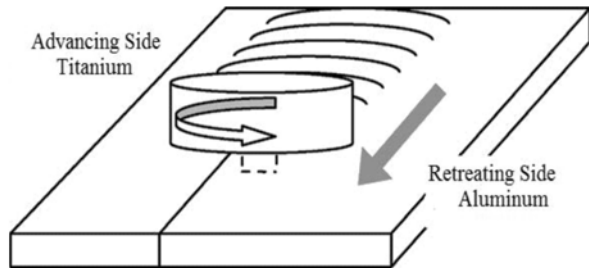
Fig. 2. Schematic of FSW process used in this research [4].
