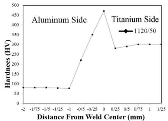
Fig. 6. Hardness profile in the butt connection of pure titanium and aluminum alloy 5083 created by friction stirring.
